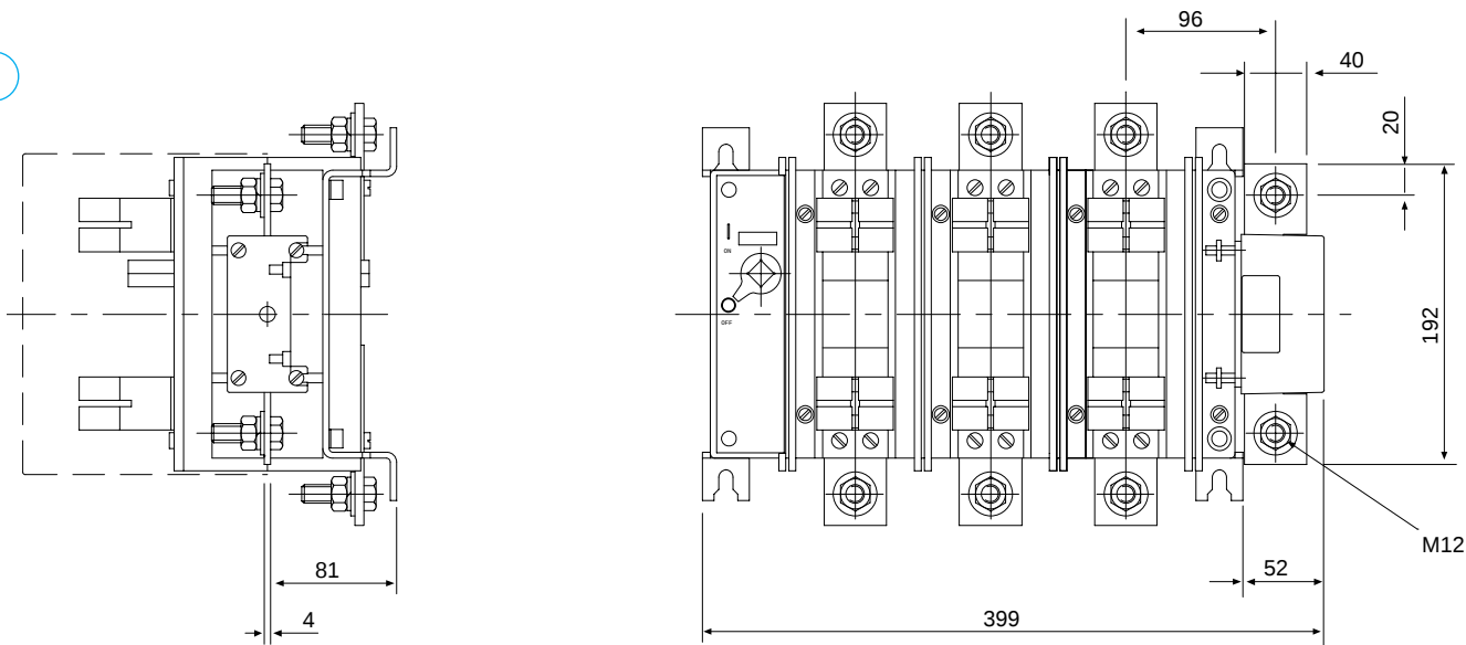
Dimensions (mm) Switched neutral type QSA 400 - QSA 800 (BS), frame size 3
