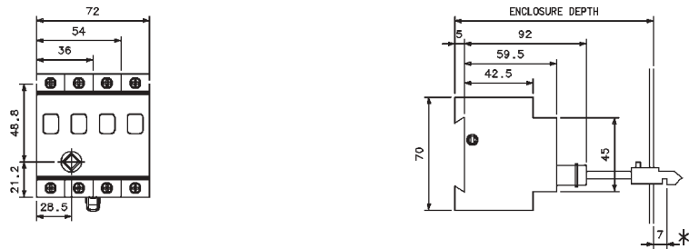
Dimensions (mm) 1) Type DMV 125 A & 160 A
