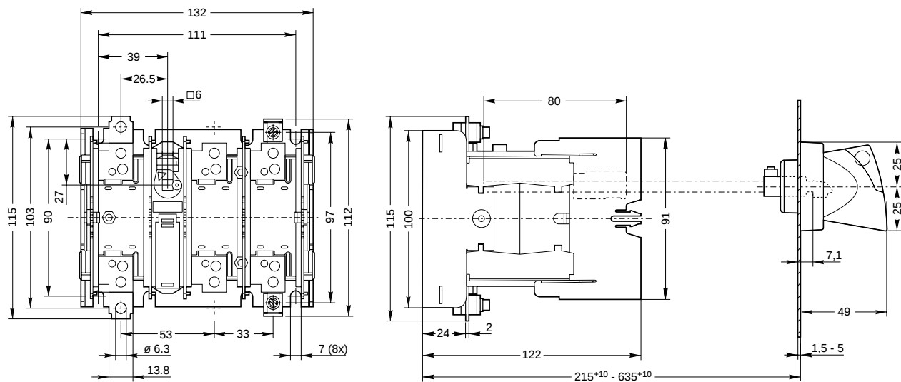
Dimensions (mm) Type QSA 40N0 - QSA 63N0 (BS), frame size 0
