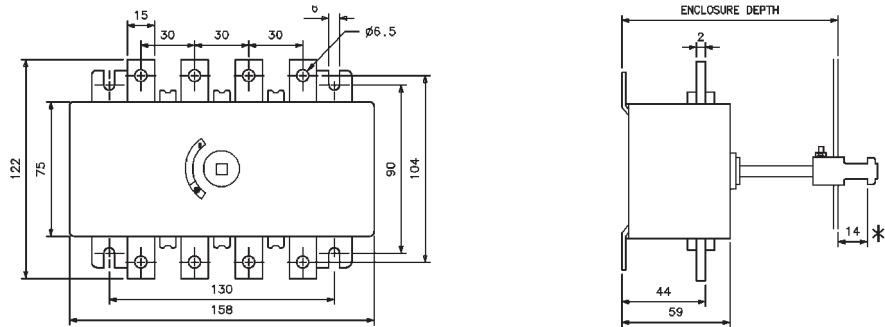
Dimensions (mm) 1) Type DMV 250 A – 1000 A
