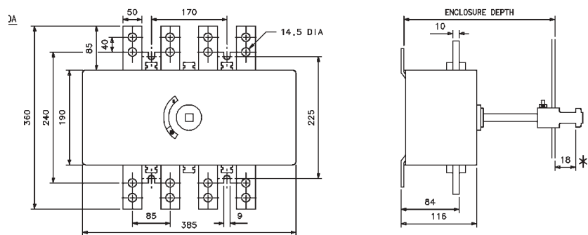
Dimensions (mm) 1) Type DMV 1600 A
